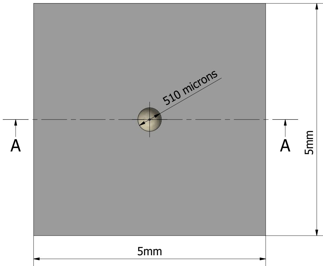
Top View ( 20 : 1 )
